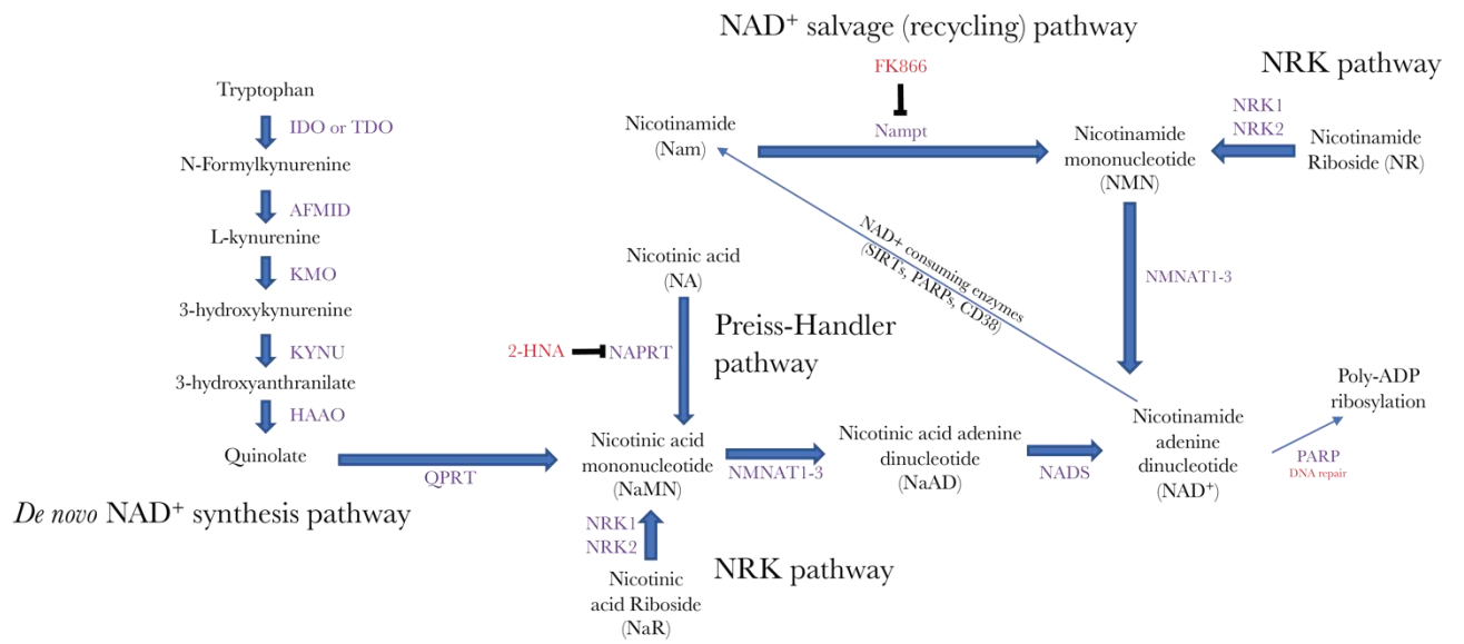
Supplemental Figure S6. Related to Figure 4 and Supplemental Figure S5. Scheme for NAD + biosynthetic pathways.
